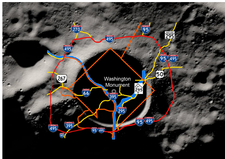
This image of Shackleton Crater on the lunar South Pole was captured by the Lunar Reconnaissance Orbiter. Laid on top is the 64-mile long Washington, D.C. Capital Beltway for scale.
